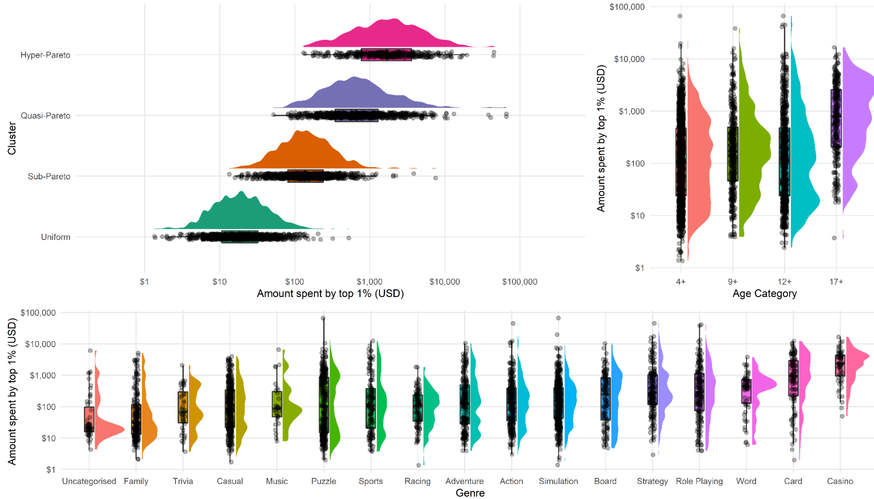
Fig. 1. Raincloud plots showing the distribution of spending amongst the top 1% of spenders within all 2,873 games in the sample, split by cluster, age category, and genre. A logarithmic transformation is applied to the y-axis to allow the visualisation of all spending. Each data point represents a single game: For example, the most extreme adventure game has 1% of its spenders invest more than $10,000 each; the least extreme has them invest less than $10.
